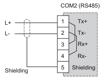
COM2 connector
