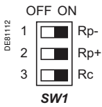
Converter positioned at end of bus
