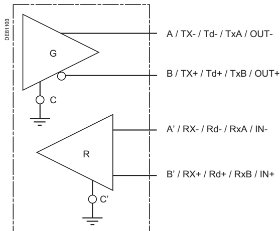
4-wire network.
