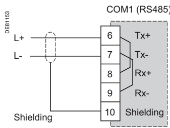
COM1 connector
