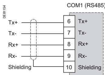
COM1 connector
