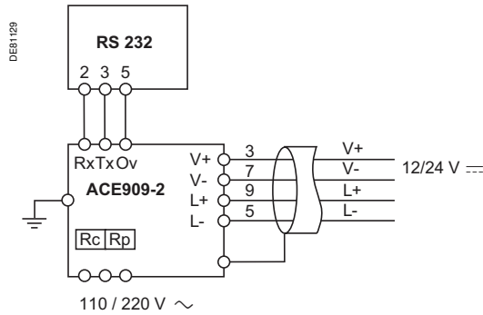
Converter not positioned at end of bus
