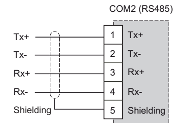
COM2 connector
