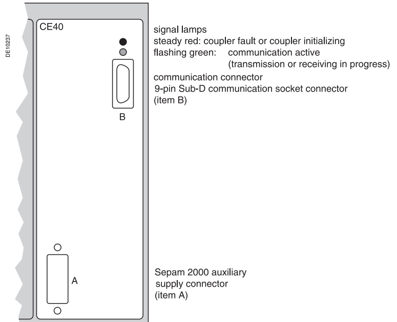
Diagram of the communication coupler board for 2-wire or 4-wire RS 485 networks
